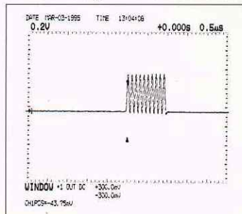
Positive-going noise
